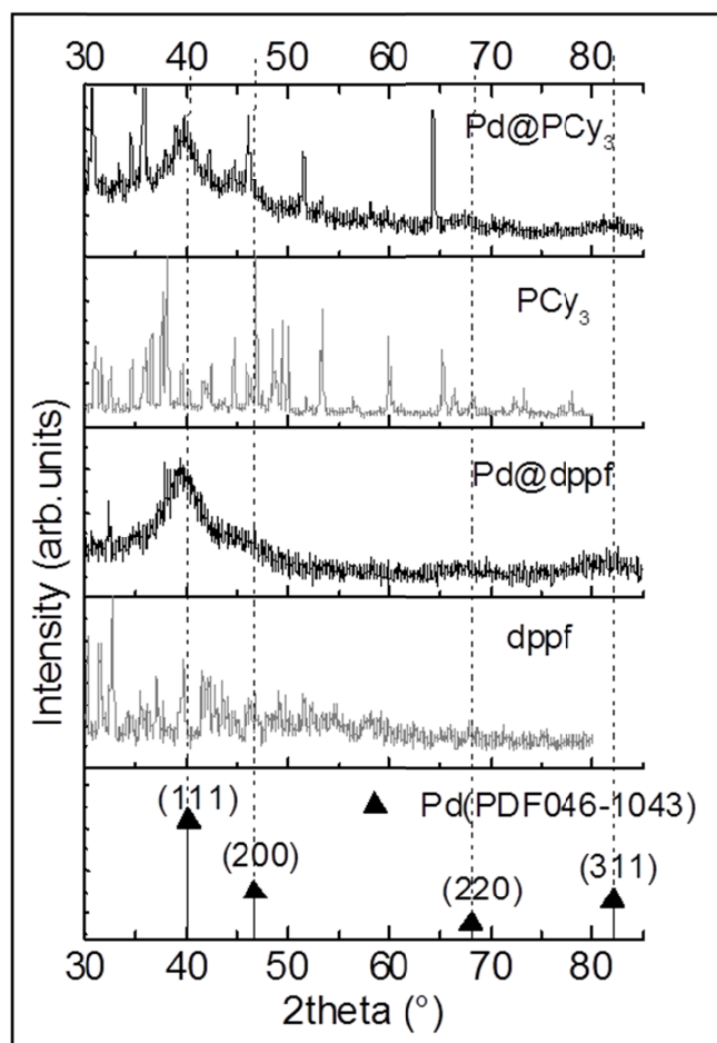
Figure S1: Powder XRD diffraction patterns of \text{Pd}@dppf and \text{Pd}@PCy_3 systems in comparison with bulk Pd and free ligands, dppf and PCy_3 .
