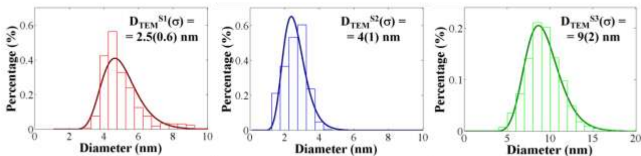
Figure Sup1. Histograms (bars) of the NP diameter, extracted from the HRTEM images, together with log-normal distribution fits (lines), providing mean particle sizes and standard deviations, D_{\text{TEM}}(\sigma) , of 2.5(0.6), 4(1) and 9(2) nm for S1 (left), S2 (center) and S3 (right), respectively.
