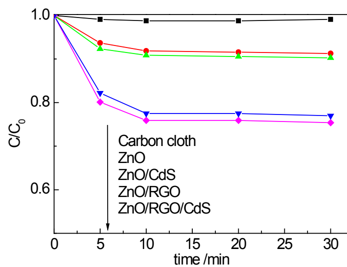
Fig. S2 MB adsorption of carbon cloth, ZnO, ZnO/RGO, ZnO/CdS and ZnO/RGO/CdS photocatalysts
