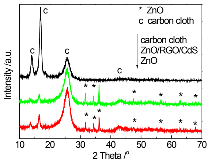
Fig. S1 XRD pattern of carbon cloth, ZnO and ZnO/RGO/CdS.
