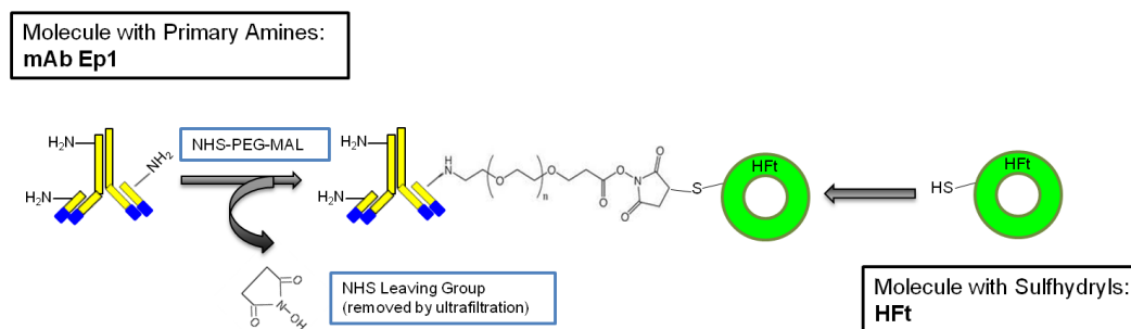
Supplementary Fig. 1: Two-step reaction scheme for the ferritin-mAb (HfT-Ep1) conjugates preparation. HfT-Ep1 was formed by reaction of NHS-PEG 3300 -MAL with amine (Ep1) and sulfhydryl (HfT) containing molecules.
