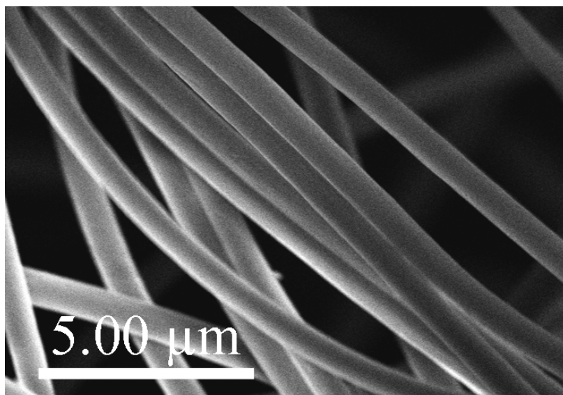
Fig. S1. FE-SEM image of the precursor of V0
