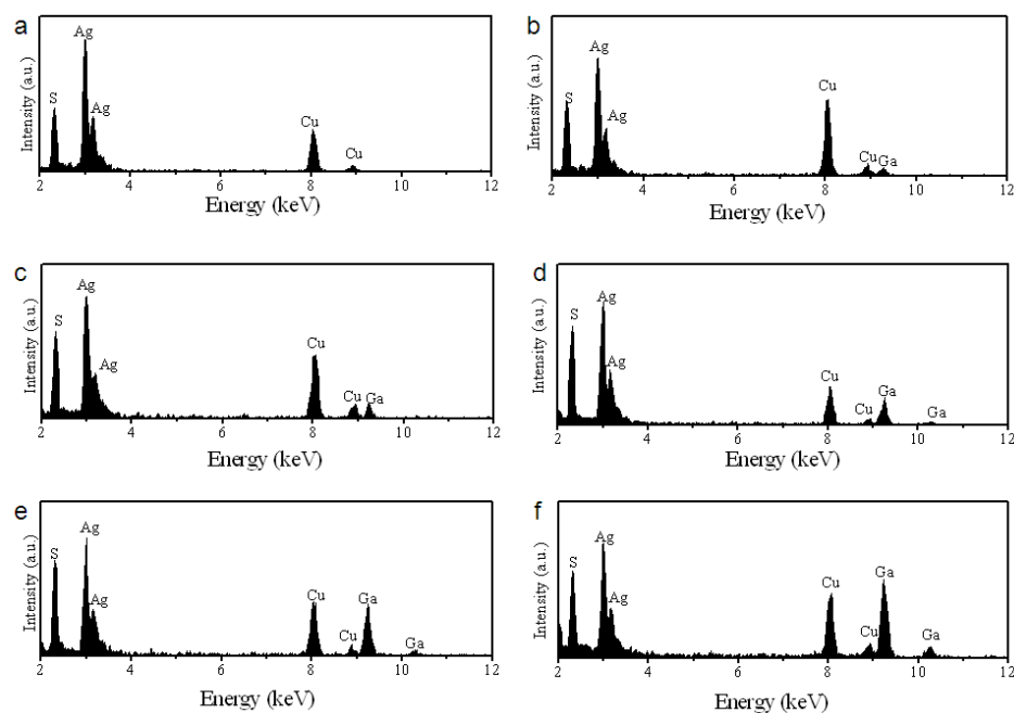
Figure S2 EDS spectra of the products having reacted for 1 min, 3 min, 5 min, 10 min, 20 min and 30 min respectively; the Cu signal comes from the copper grid.
