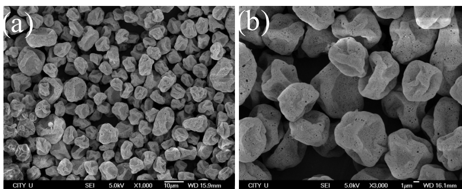
Fig. S1 SEM images of microspheres prepared from electrospraying PMMA solution without nonsolvent. The polymer concentration is 3 wt%. (a) low and (b) high magnification.
