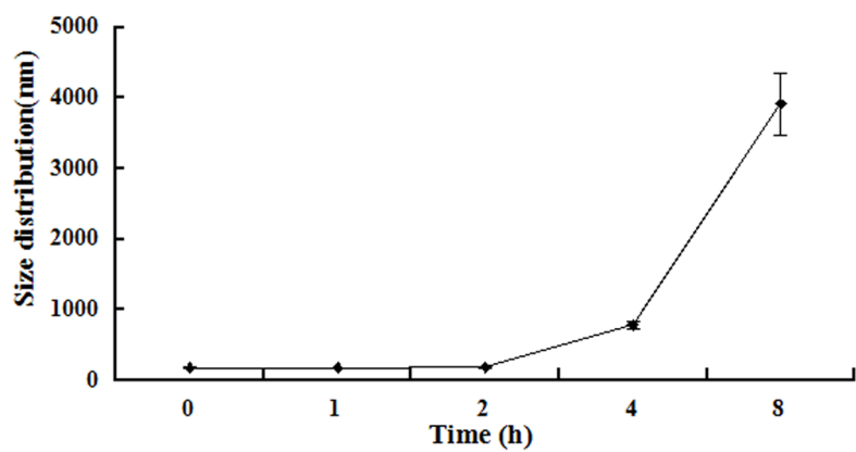
Fig. S3. The particle size changes of TPTN in the presence of 10% serum in 8 h.
