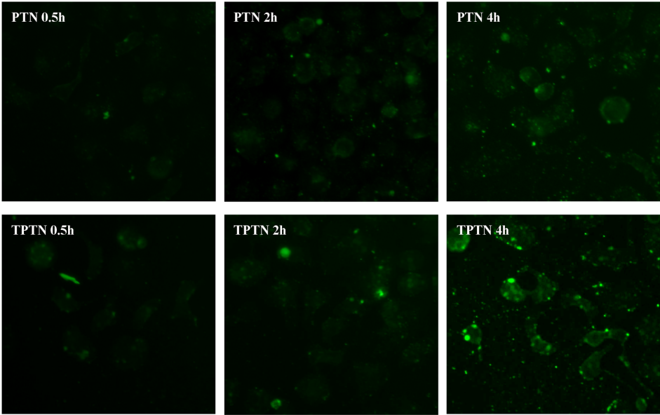
Fig. S4. Results of fluorescence microscope of the PTN and TPTN incubated with the HepG2 cells at different times
