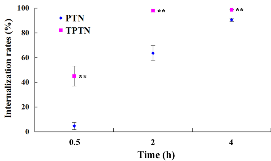
Fig. S5. Results of flow cytometry of the PTN and TPTN incubated with the HepG2 cells at different times.
