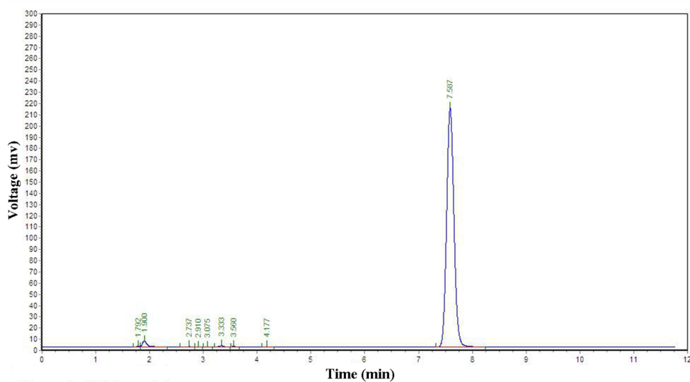
Fig. S2. The HPLC chromatogram of sorafenib.
