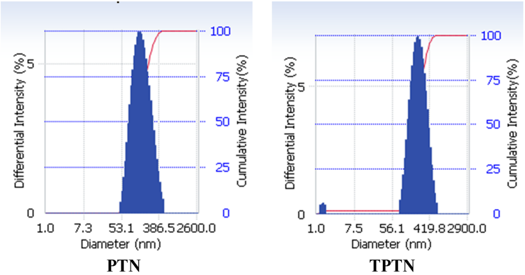
Fig. S1. Results of particles size distribution of the PTN and TPTN.
