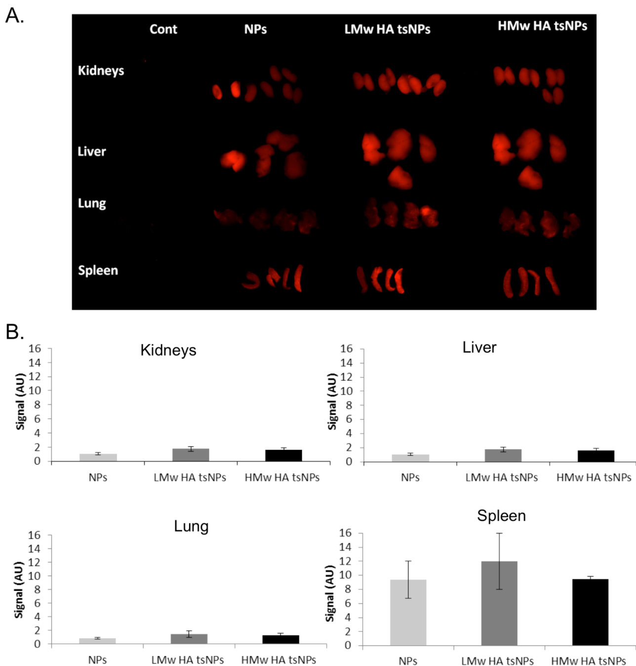
Supplementary Figure 1: Biodistribution of NPs and tsNPs in B16F10 SC tumor bearing mice. Mice were injected with PBS, Cy5 labeled NPs or tsNPs. 3.5 hours post injection mice organs were isolated and fluorescent signals were measured as described in the experimental section. A. Isolated organs B. The scaled fluorescent signal levels per area of isolated organs were measured by Maestro in vivo fluorescence imaging system.
