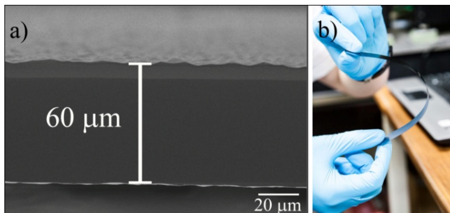
Fig. S1. (a) SEM image of etched thin Si wafer which have a thickness of 60 \mu\text{m} (b) The bending flexibility is demonstrated by hands.
