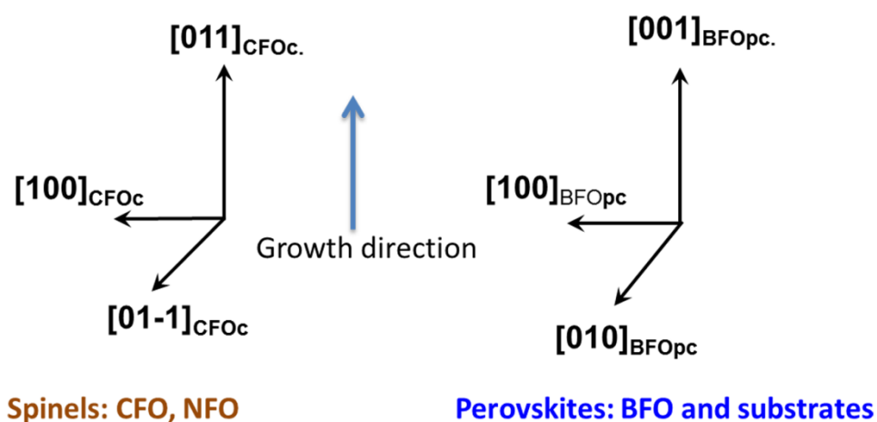
Fig. s1 A schematic of 3-d relationships in the perovskite-spinel systems.
