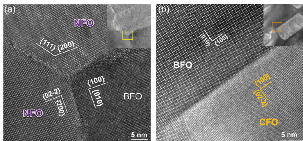
Fig.s2 Plan-view hrtem from bfo[001] and [011]nfo/cfo directions.
