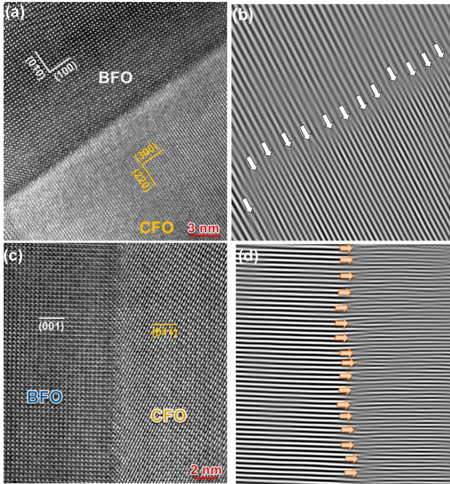
Fig. s3 The bfo-cfo interfaces with one-dimensional fft filtered images, (a) and (b) plane-view, (c) and (d) cross-section.
