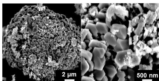
Fig. S2 SEM images of \text{LiMn}_2\text{O}_4 synthesized from the \text{Mn}_2\text{O}_3 precursor.
