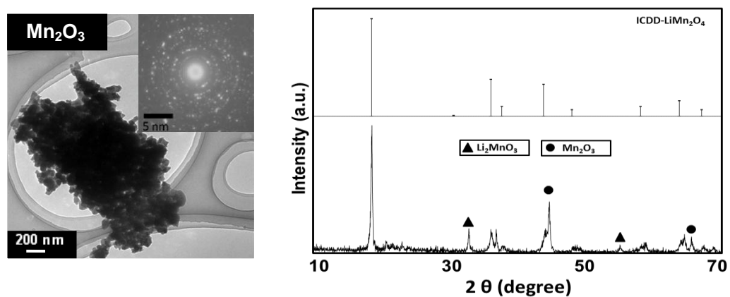
Fig. S1 TEM image and XRD pattern of \text{Mn}_2\text{O}_3 prepared from the \text{MnCO}_3 precursor.
