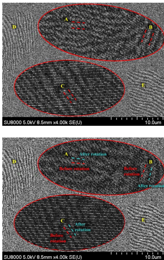
Figure S Rotation directions of the secondary Moiré fringes on the alumina nanoporous structure when the digital gratings are anticlockwise rotated, (a) before rotation and (b) after rotation.
