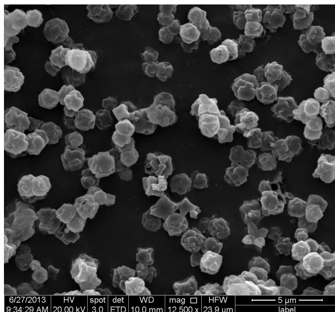
Fig. S2 SEM image of the obtained hollow CeO 2 nanocubes.
