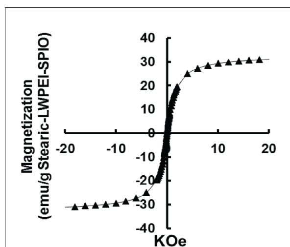
Supplementary Fig. S1 Magnetic hysteresis loop of Stearic-LWPEI-SPIO nanoparticles recorded at 300 K.
