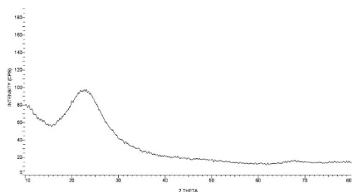
Figure S1: XRD spectrum illustrating the amorphous nature of the mesoporous silica nanoparticles
