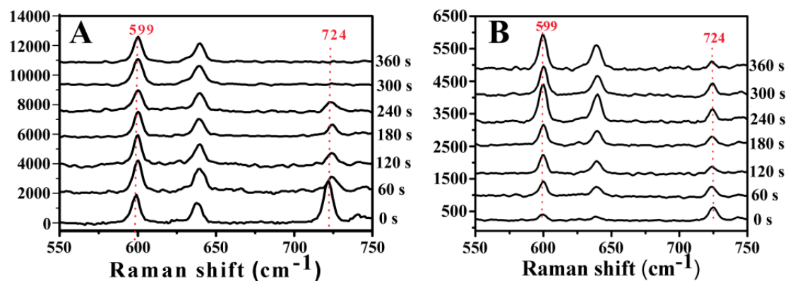
The enlarged peaks at area 550-750 \text{cm}^{-1} of Fig. 3A and Fig. 3B
