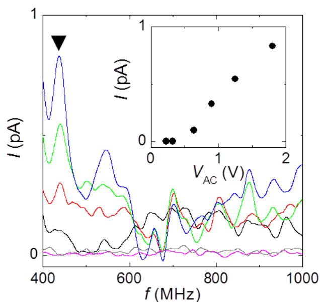
Fig. S1. The power dependence measurement of the current towards the electrode D1 at the input RF powers of 0, 3, 9, 12, 15, and 18 dBm. The inset shows the current at a specific resonance (indicated by a triangle in black). The threshold voltage is estimated to be around 0.5 V.
