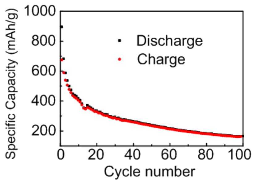
Figure S3. Cycling performance of commercial MoS 2 .
