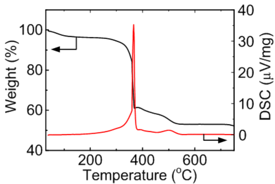
Figure S2. TGA and DSC curves of MoS 2 /OLC nano-urchins.
