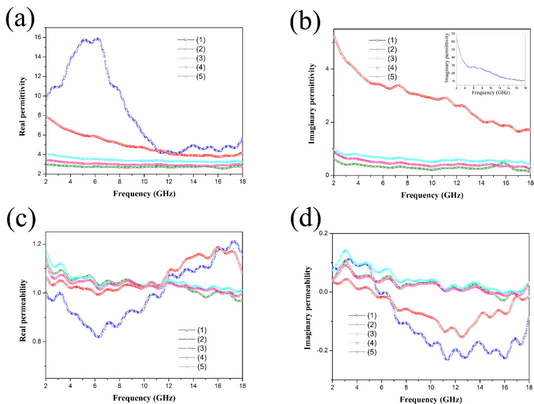
Fig. S1 Measured frequency dependence of (a) real and (b) imaginary parts of complex permittivity and (c) real and (d) imaginary parts of permeability: (1) EG, (2) HCl-PANI, (3) PANi/EG-0, (4) PANi/EG-1, (5) PANi/EG-2.
