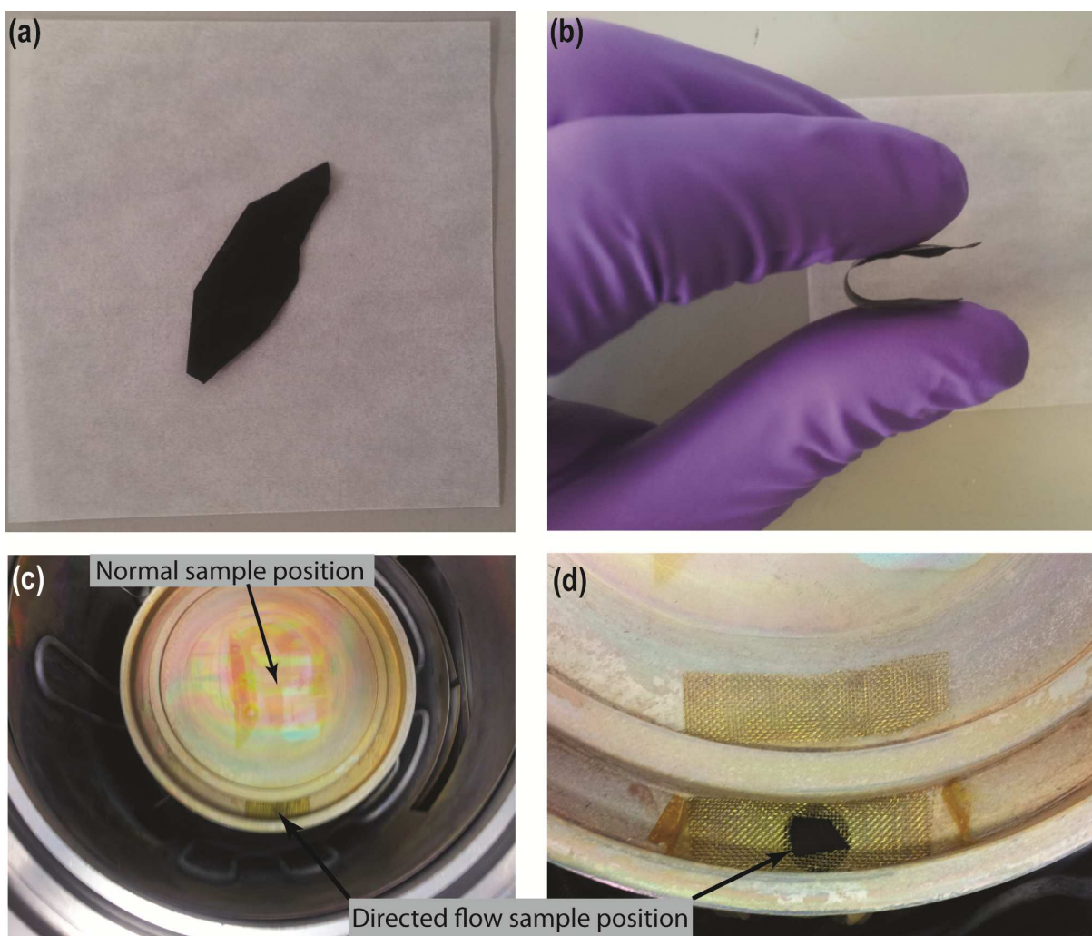
Figure S1. Photographs of a large, flexible gyroidal mesoporous resin template (a+b) and of the Beneq TFS200 ALD system used for part of the samples described in this report, indicating the sample position for the normal "flow over" and the "directed flow" procedure.
