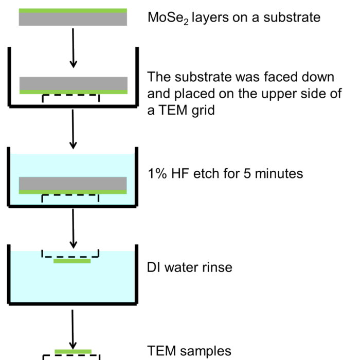
Fig. S2 A direct transfer method used for preparation of MoSe 2 TEM samples.
