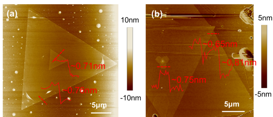
Fig. S1 AFM images and height profile of bilayer and trilayer MoSe 2 flakes.
