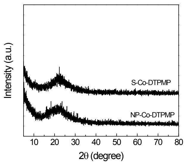
Fig. S1 XRD pattern of the synthesized cobalt phosphonate hybrid materials.
