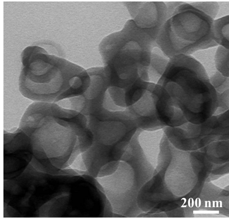
Fig. S3 TEM image of the S-Co-DTPMP sample after three times cycling test.
