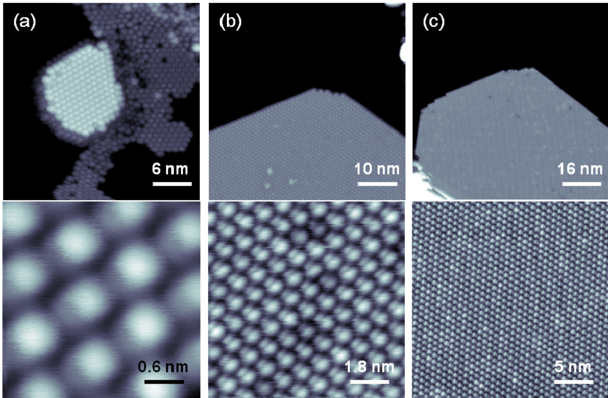
Fig. S1 Self-assembled fullerene islands of various sizes. (a) V_{sample} = 1.5 V and I_t = 50 pA, (b) V_{sample} = 2.0 V and I_t = 50 pA, and (c) V_{sample} = 1.5 V and I_t = 50 pA. The bottom images are magnified images of the upper ones.
