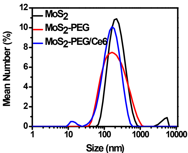
Supporting Figure S1. DLS measured hydrodynamic sizes of MoS 2 nanosheets before & after after PEGylation or Ce6 loading.
