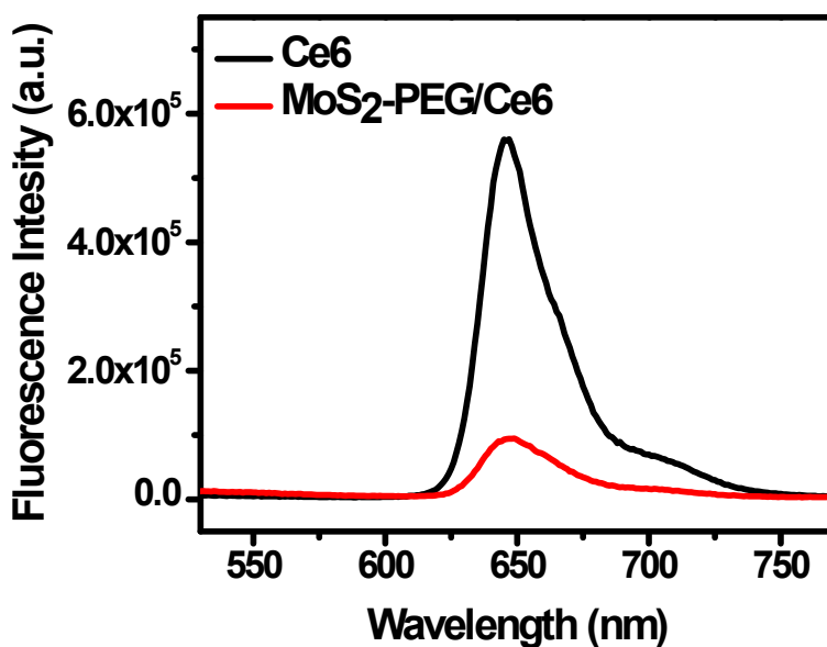
Supporting Figure S2. Fluorescent spectra of Ce6 and MoS 2 -PEG/Ce6 aqueous solutions at the same Ce6 concentration ( \lambda_{ex} = 404 nm), demonstrating fluorescence quenching of Ce6 after loading onto MoS 2 -PEG.
