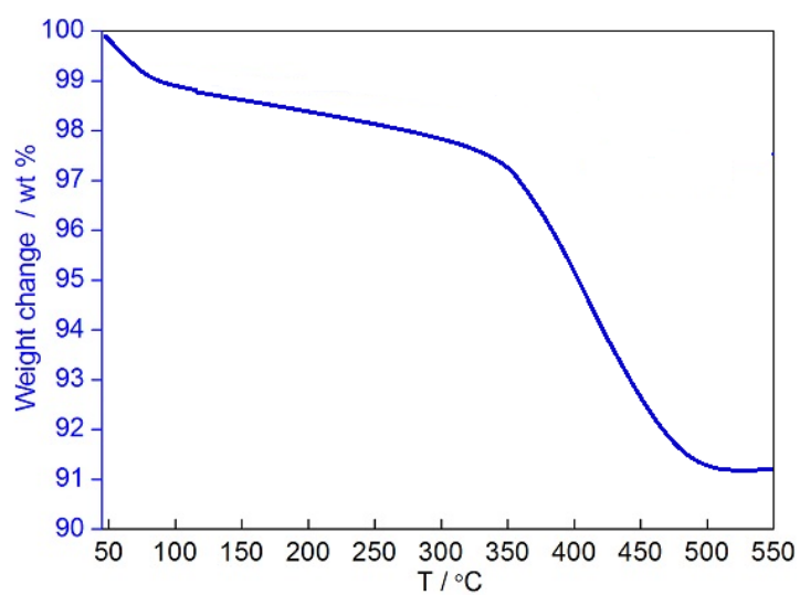
Fig. S1 TG analysis of the carbon content of the prepared \text{CoFe}_2\text{O}_4 nanocubes sample after calcinations.
