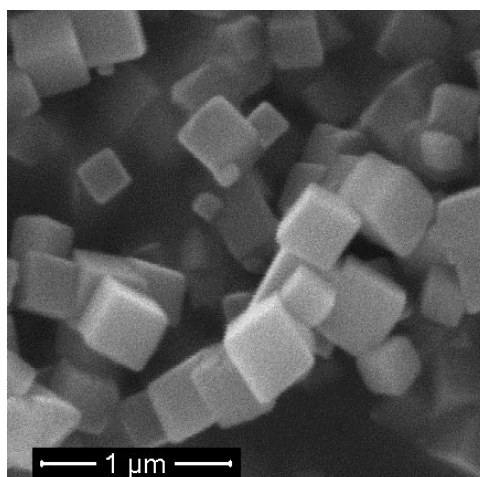
Fig. S4 SEM image of as-synthesized hollow \text{ZnCo}_2\text{O}_4 nanocubes.
