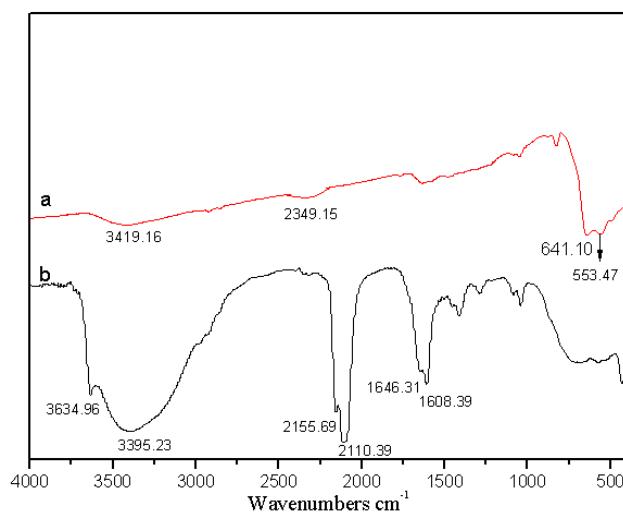
Fig. S2 FTIR spectra of hollow \text{CoFe}_2\text{O}_4 nanocubes and its precursor corresponding to curve a and b, respectively.
