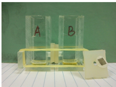
Figure S1 A photograph of the inter-diffusing cell and a nano-porous MWCNT membrane with Au-nanorods inside of CNTs.
