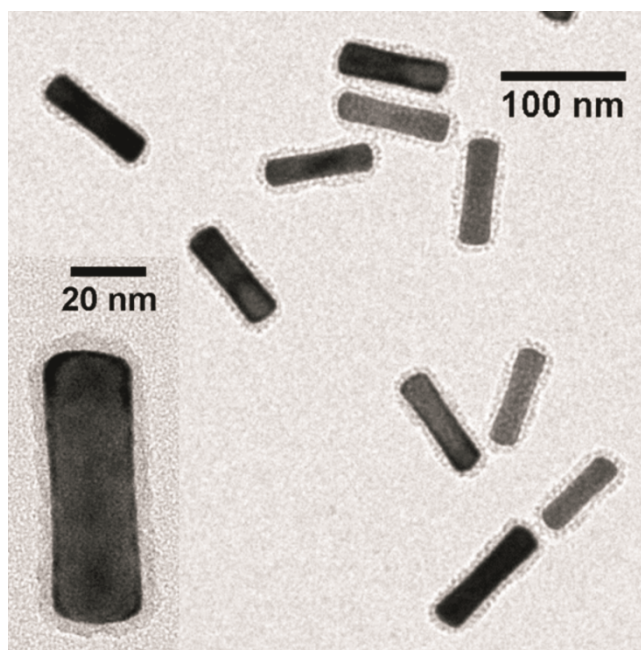
Figure S1. TEM image (at low and high magnifications) of PEGylated silica-coated GNRs used in this study
