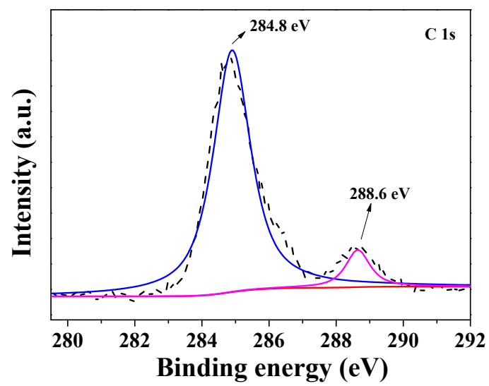
Figure S1 XPS spectrum of C 1s for the as-synthesized 1.5Ag-N-TiO 2 -YSM.
