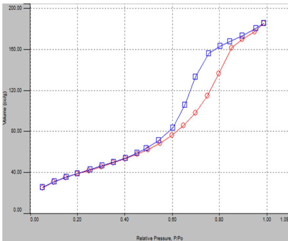
Figure S4 N 2 adsorption-desorption isotherms of the reused 1.5Ag-N-TiO 2 -YSM.
