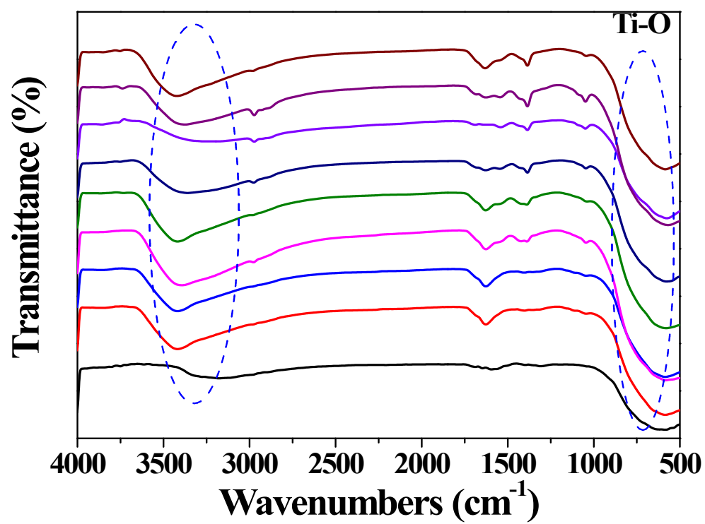
Figure S2 FTIR spectra of N-TiO 2 -YSM and a series of Ag-N-TiO 2 -YSM.
