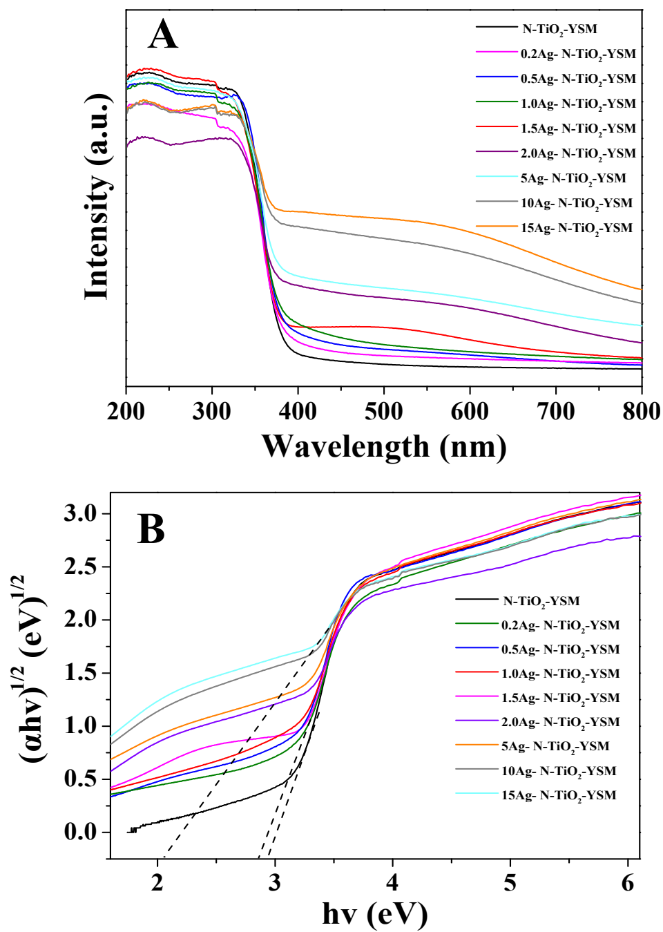
Figure S3 UV-vis diffuse reflectance spectra (A) and the band-gap energies (B) of as-prepared TiO 2 -based materials.
