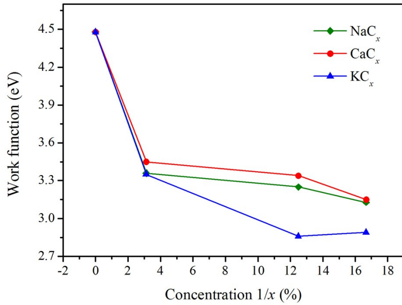
Fig. S3 Work function variation of MC x with respect to the concentration 1/x.
