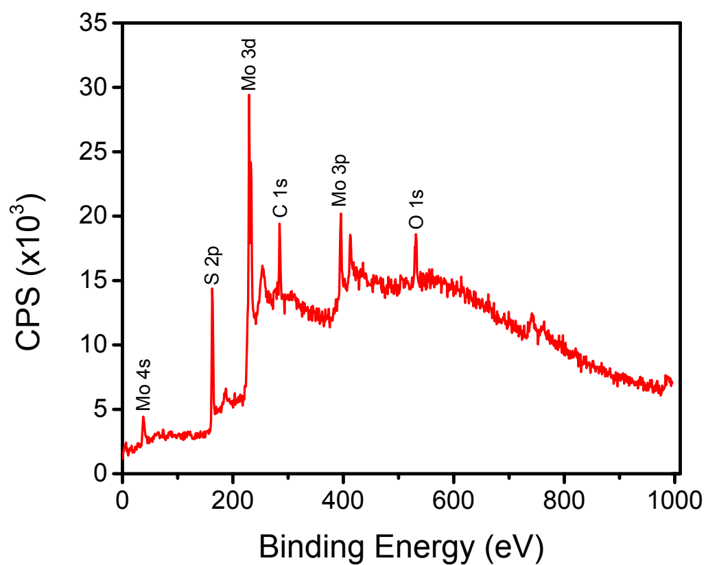
Figure S1. Survey X-ray photoelectron spectrum of MoS 2 after exfoliation. Mo and S signals originate from MoS 2 while C and O from the sample holder. Note the absence of Li 1s signal at ~55 eV.
