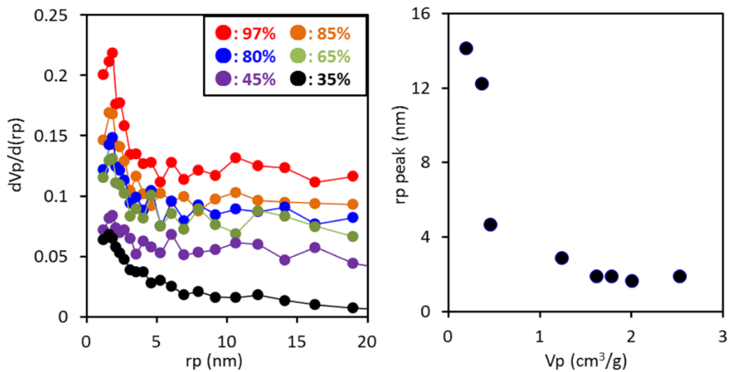
Fig. S1 The pore size distribution estimated by Barrett-Joyner-Halenda (BJH) method from nitrogen adsorption isotherms. The pore size distribution showed a monotonic decrease as the purity decreased.
