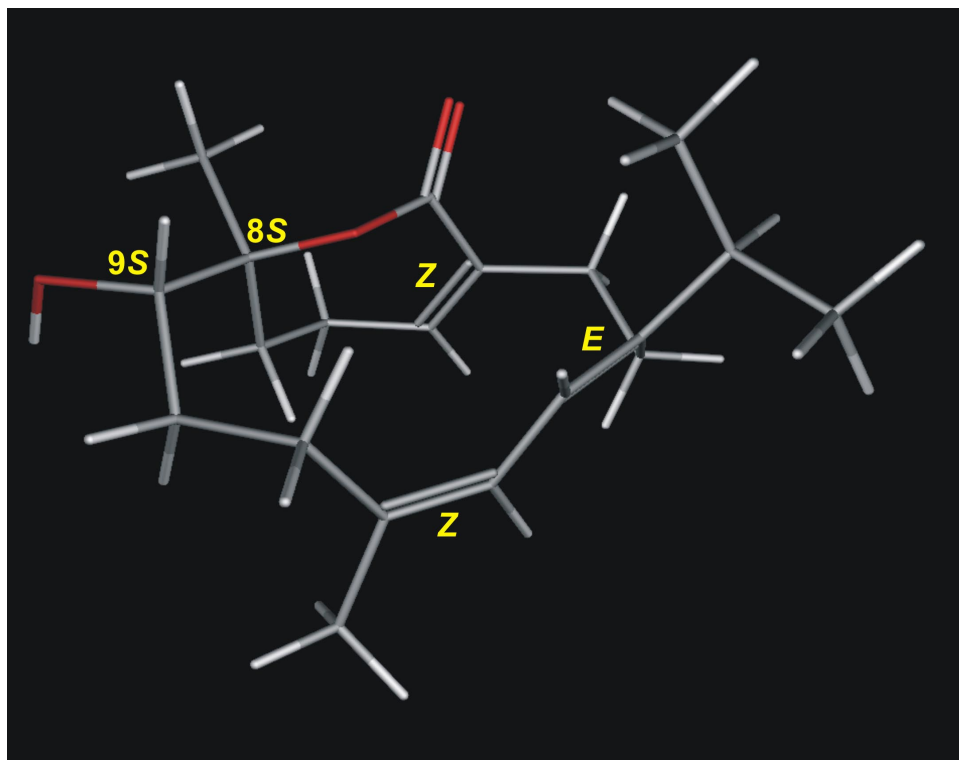
Minimum energy conformation of compound 1 shown from a different perspective than in Fig. 3.
