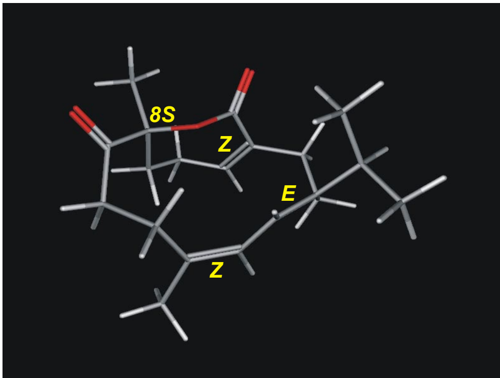
Minimum energy conformation of compound 2
