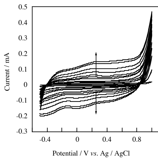
Supplementary Fig. 1 CV for formation of SWNTs•DNA/poly(EDOT) composite film: 50 \text{ mmol dm}^{-3} LiCl aqueous solution, under argon atmosphere, scan rate 50 \text{ mV s}^{-1} , 25 \text{ }^\circ\text{C} .
