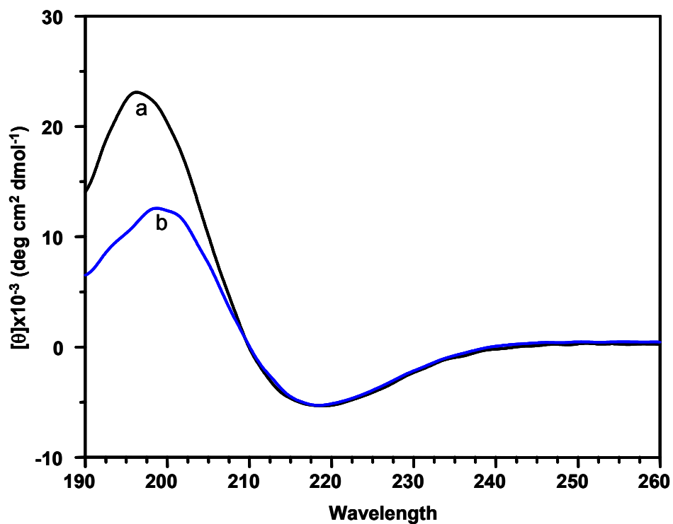
a) Normal CD spectrum of PrP[Ac-106-126-NH 2 ] recorded in SDS 5x10 -3 M, b) CD spectrum of the same sample obtained with the cuvette in contact with the photomultiplier window.
