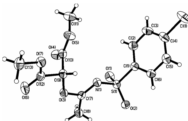
Fig. S2 X-Ray crystal structure of (dimethoxycarbonyl)-methylester of N -( p -Cl-benzenesulfonyl)imidoylacetic acid 5b
