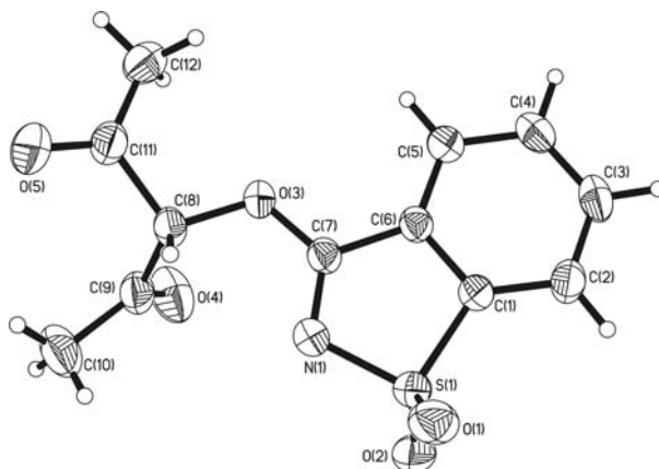
Fig. S1 X-Ray crystal structure of 3-(diacetyl)-methoxybenzo[ d ]isothiazol 1,1-dioxide 4c
