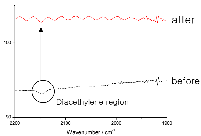
Fig. S2. IR Spectra of the hydrogel 1 before and after UV polymerization.
