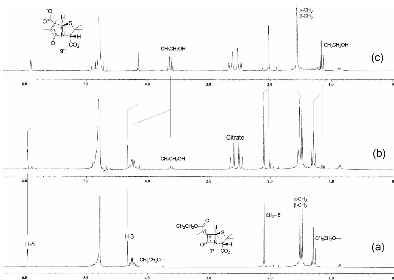
Figure S1. ^1\text{H} NMR spectra of (a) 7' in \text{D}_2\text{O} buffer (0.02 M phosphate, pH 7.2, 25 °C), and (b) 26 min, (c) 3.5 h following addition of \beta -lactamase enzyme in a citrate buffer.
