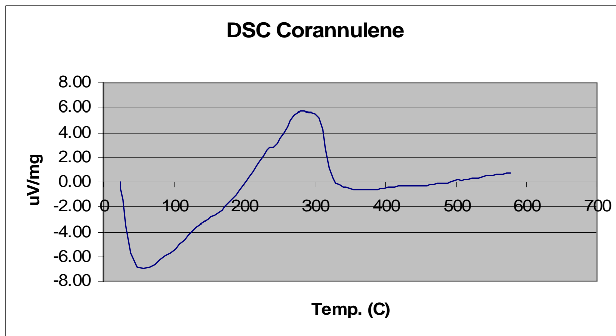
DSC of Corannulene (1)
