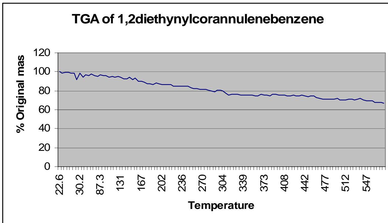
TGA of 1,2 diethynylcorannulenebenzene (5)
