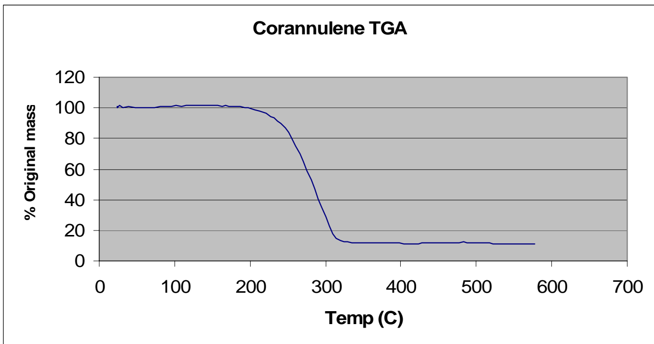
TGA of Corannulene ( 1 )
