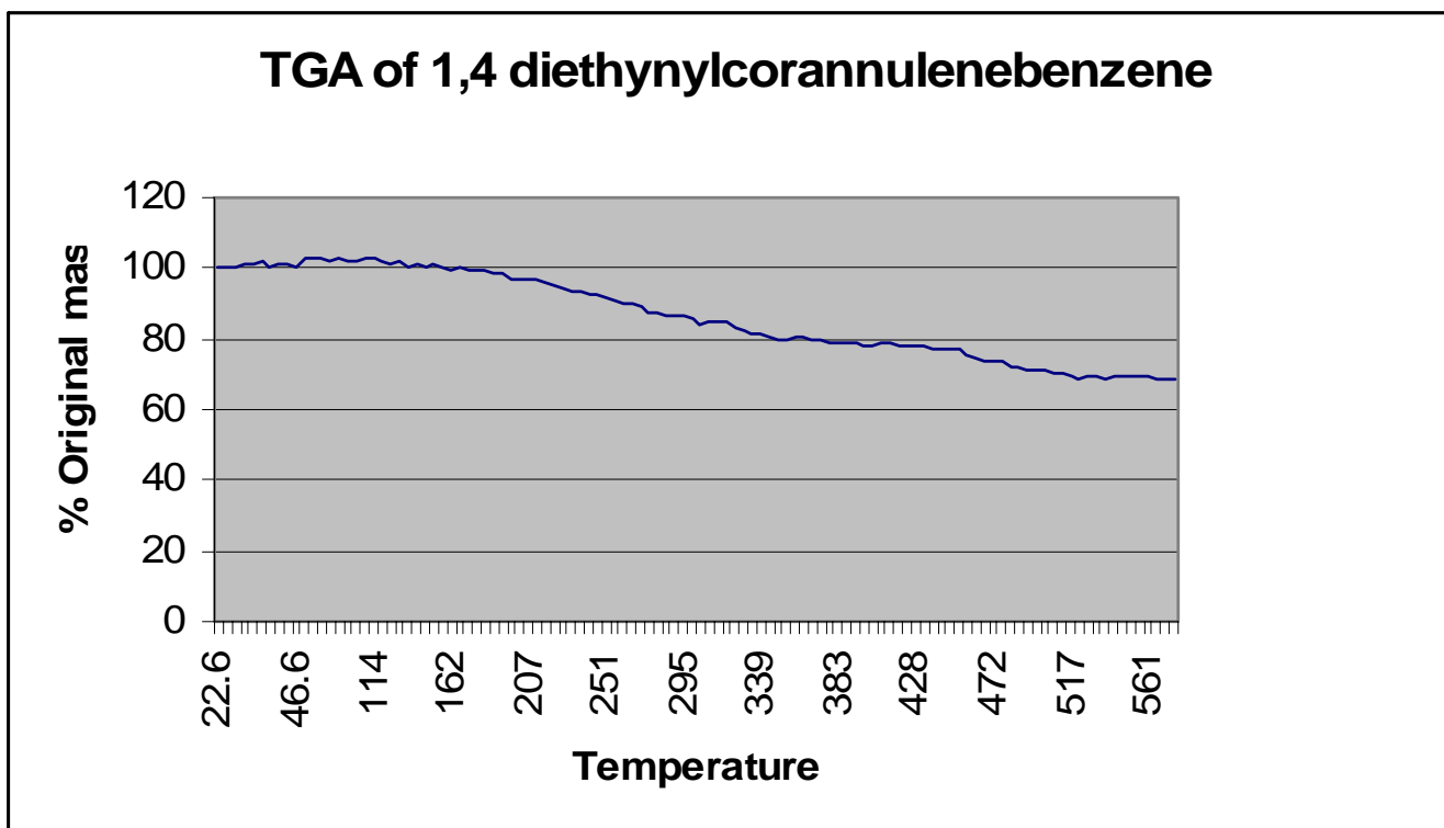
TGA of 1,4-diethynylcorannulenebenzene (6)
