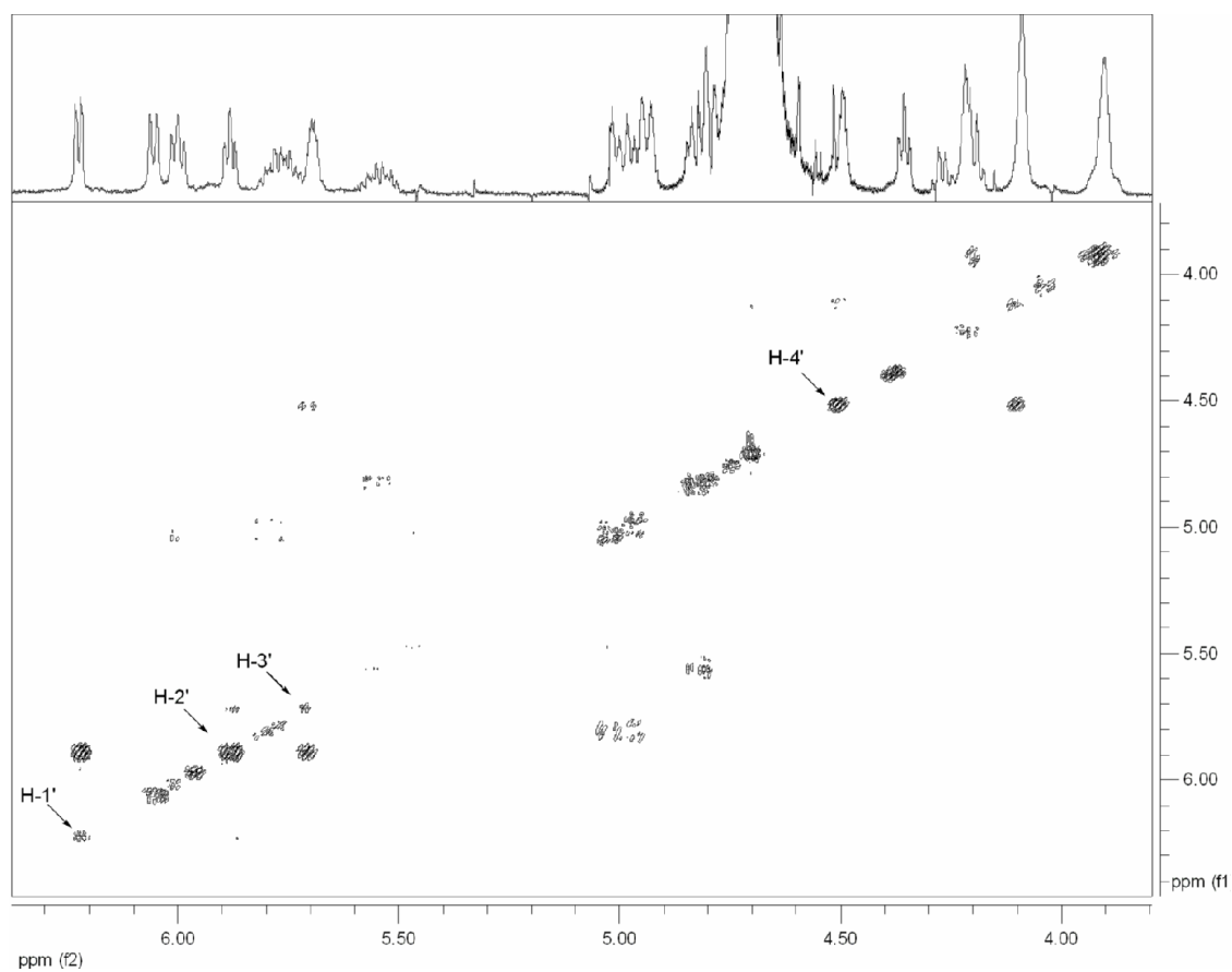
Figure S2. gDQCOSY spectrum of 2'- O -[ N -(4-pentenoyl)-( S )-alanyl]-3'- O -[ N -(4-pentenoyl)-( S )-[1- ^{13}\text{C} ]valyl]-pdCpA (6.3 ppm to 3.8 ppm) with ^1\text{H} spectrum shown on horizontal axis.
