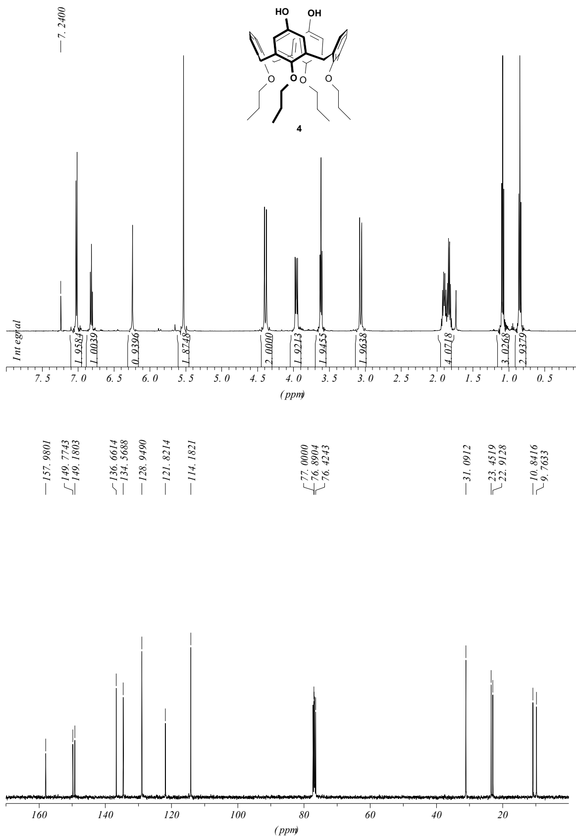
Fig. S1 ^1\text{H} and ^{13}\text{C} NMR spectrum of 4 in \text{CHCl}_3 .
