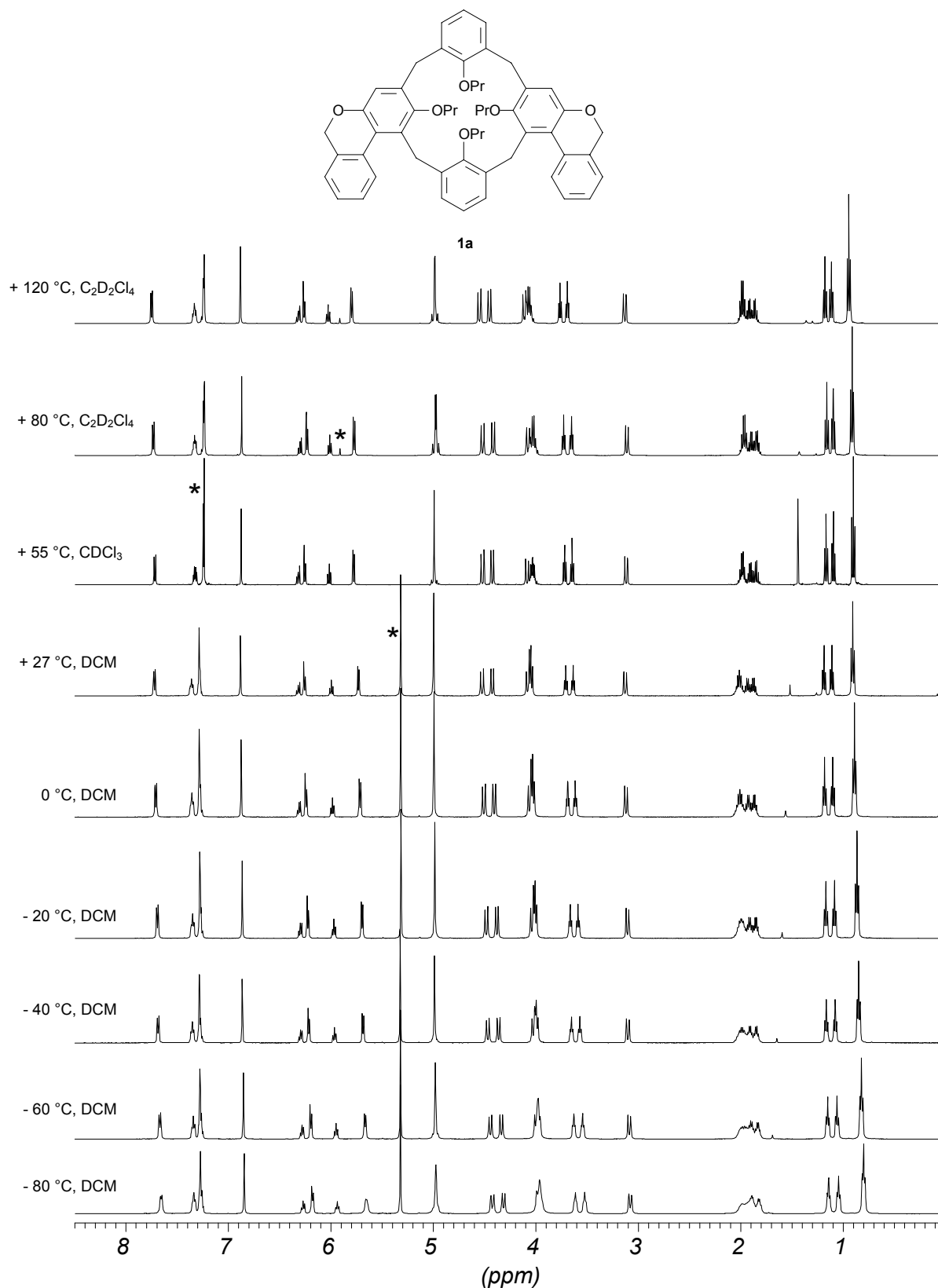
Fig. S3 Variable temperature ^1\text{H} NMR spectra 1a , residual solvent signals are marked (*).
