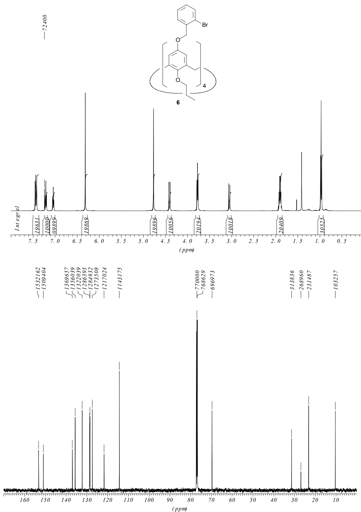
Fig. S8 ^1\text{H} and ^{13}\text{C} NMR spectrum of 6 in \text{CHCl}_3 .
