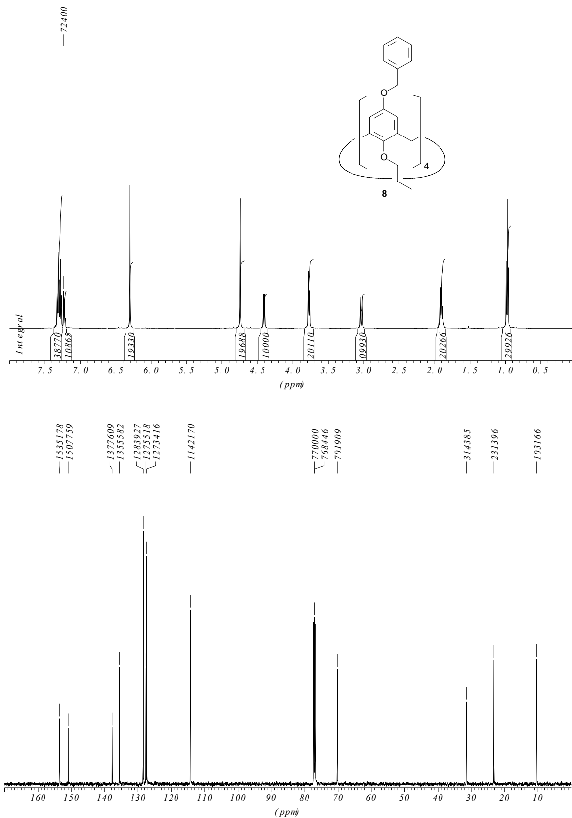
Fig. S7 ^1\text{H} and ^{13}\text{C} NMR spectrum of 8 in \text{CHCl}_3 .
