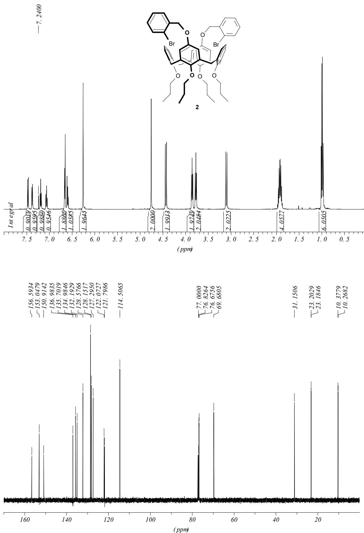
Fig. S2 ^1\text{H} and ^{13}\text{C} NMR spectrum of 2 in \text{CHCl}_3 .
