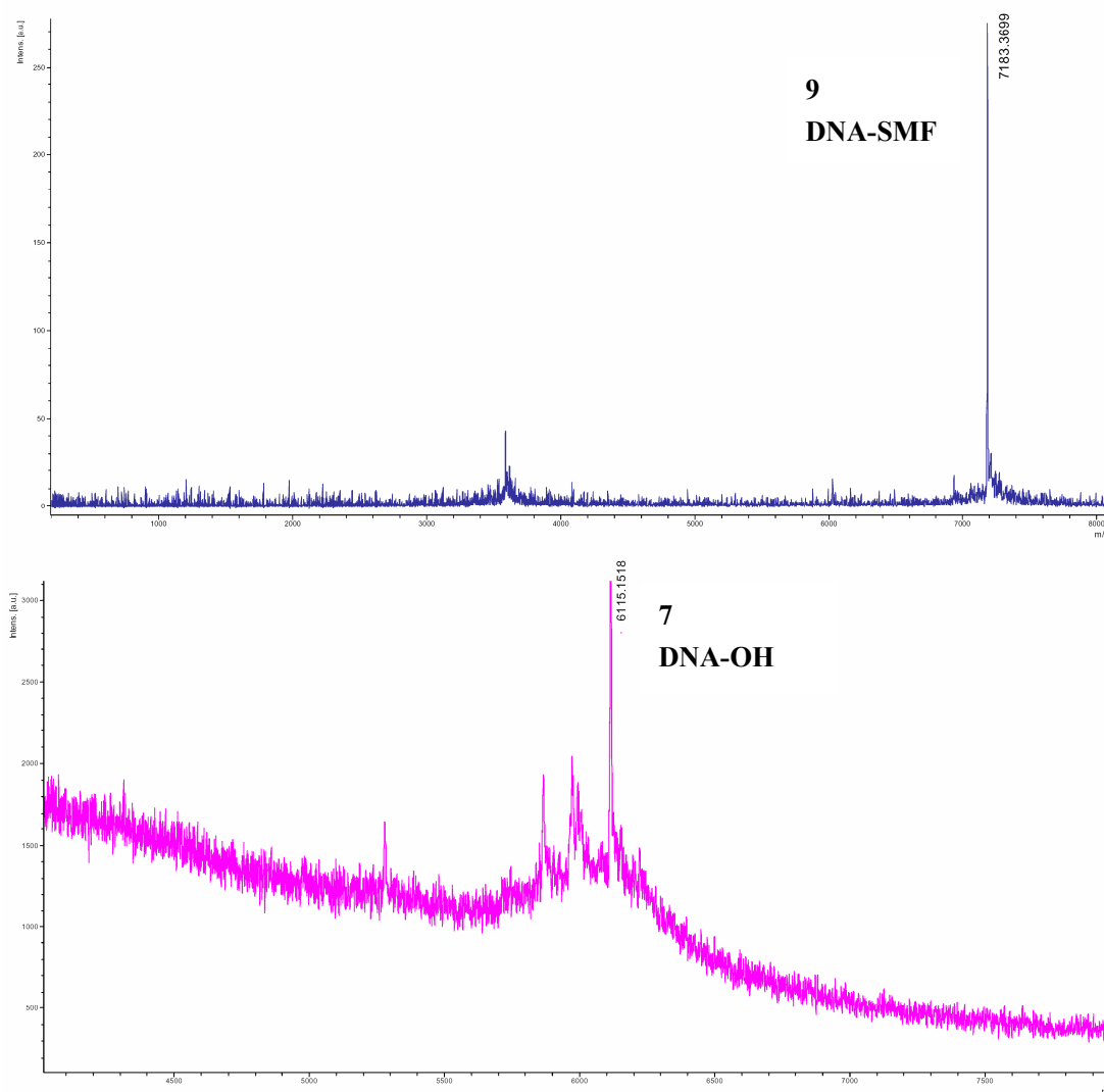
Figure S2. MALDI-TOF spectra of compounds 5-9 . (Matrix: 3-hydroxypicolinic acid)
