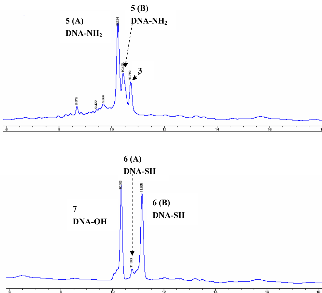
Figure S1. (A) HPLC Spectrum of DNA-NH 2 (5), (B) of DNA-SH (6) prepared
