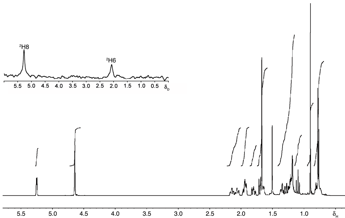
Figure S1: ^1\text{H} NMR spectrum of (+)-aristolochene isolated from incubation of PR-AS and FPP. Inset: ^2\text{H} NMR spectrum of aristolochene isolated from incubation of PRAS and FPP in ^2\text{H}_2\text{O} .
