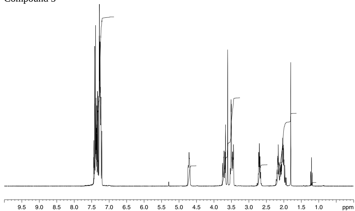
Compound 3
