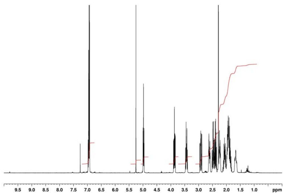
Compound 5a
