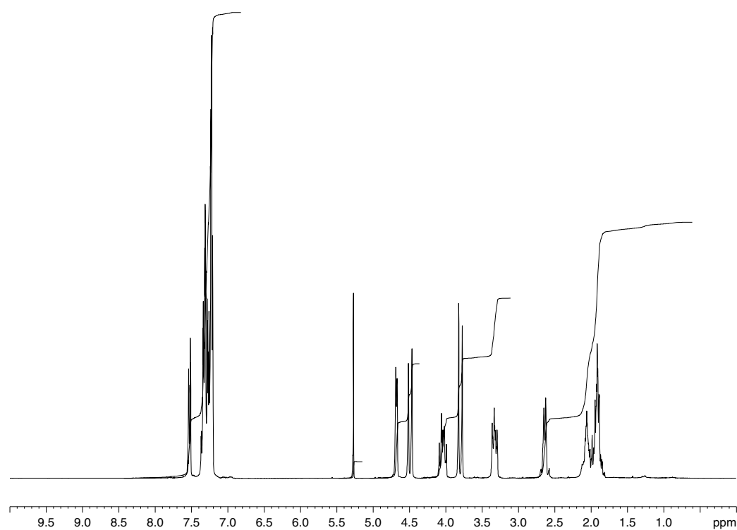
Compound 12a
