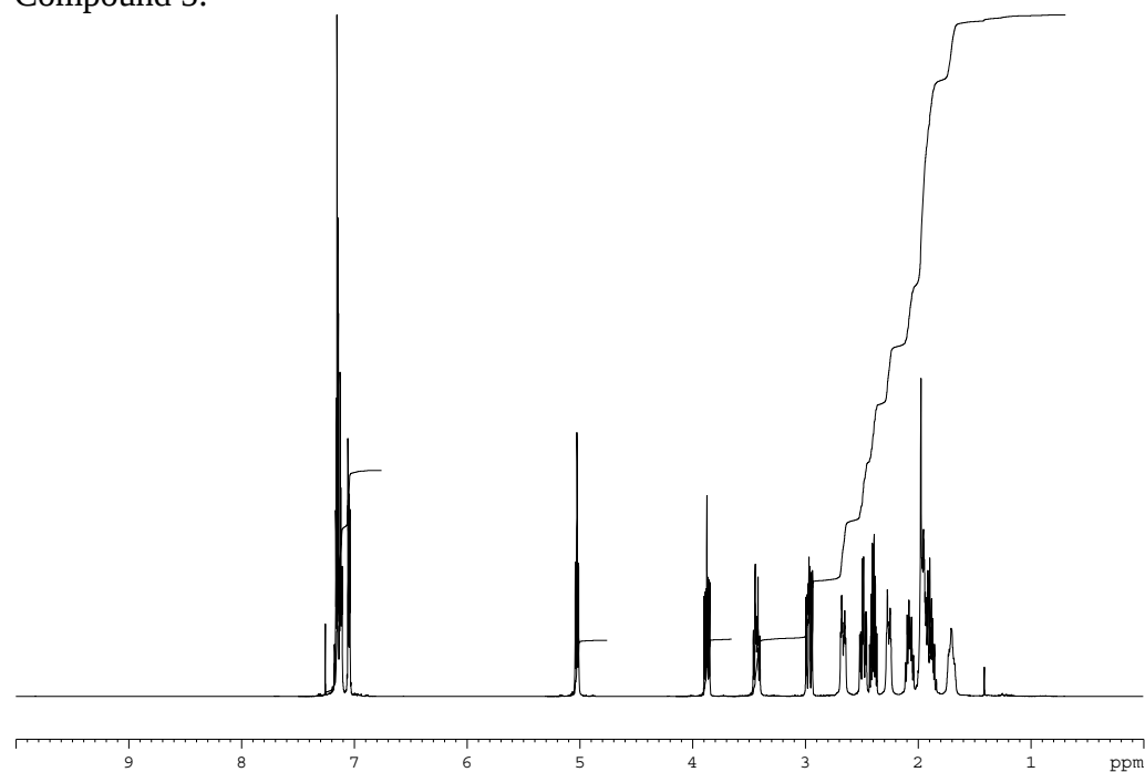
Compound 5:
