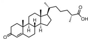
1a (25 R )- \Delta^4 -Dafachronic acid
