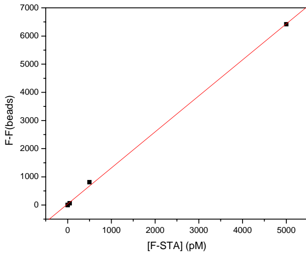
Figure S2. Calibration curve for the determination of the concentration of binding sites for spore.
