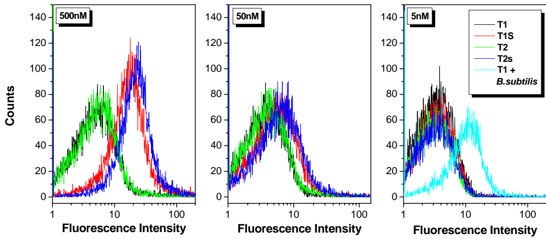
Figure S1. Binding of the different tetraivalent peptides to B. licheniformis spores at different concentrations of peptides.
