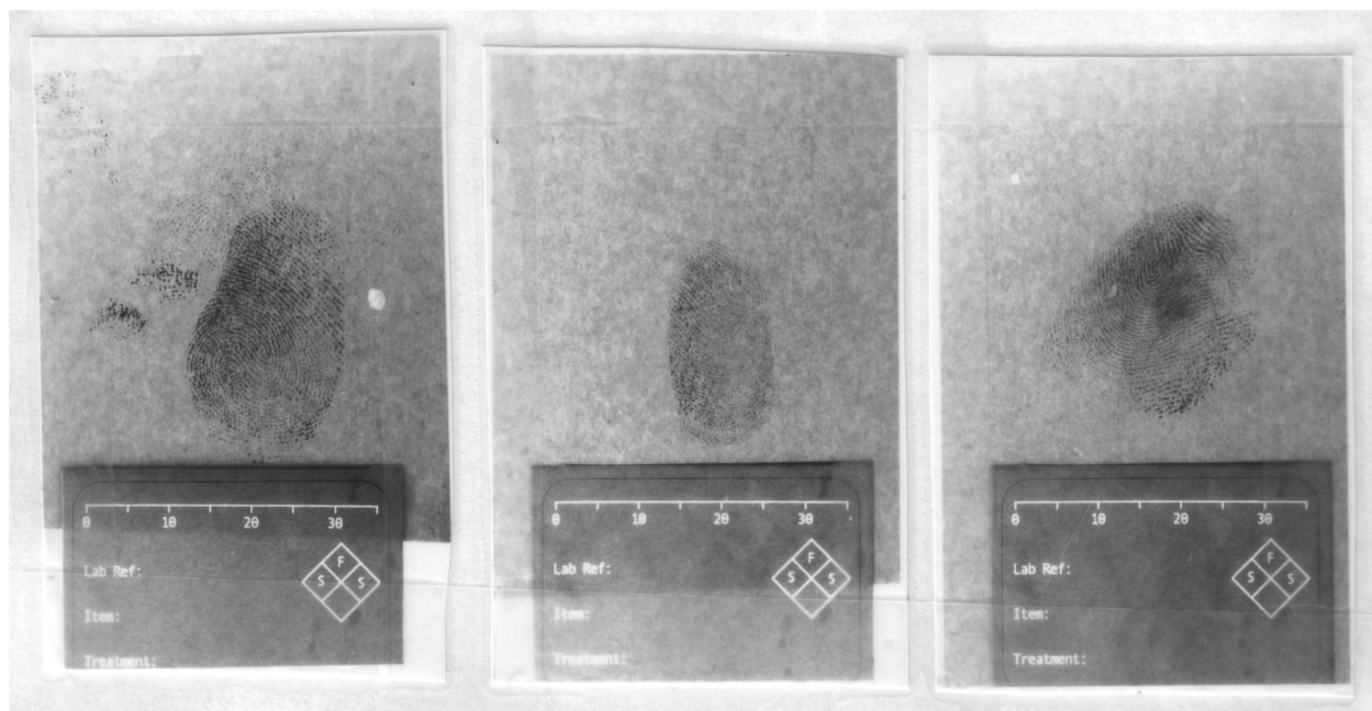
Photographs Fingerprints developed using N-methylpyridine-4-carboxaldehyde iodide 9
