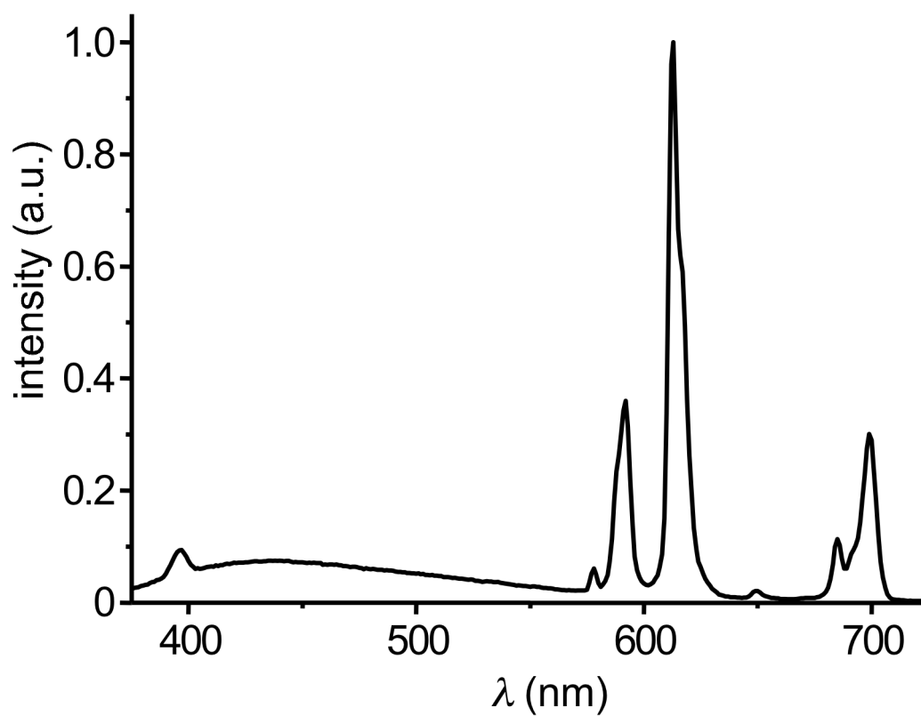
[Eu( 7a )] luminescence spectrum
