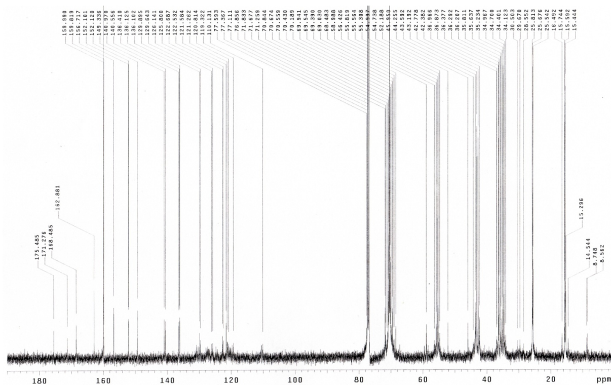
Figure S10. 13 C NMR of compound 2 in CDCl 3 .
