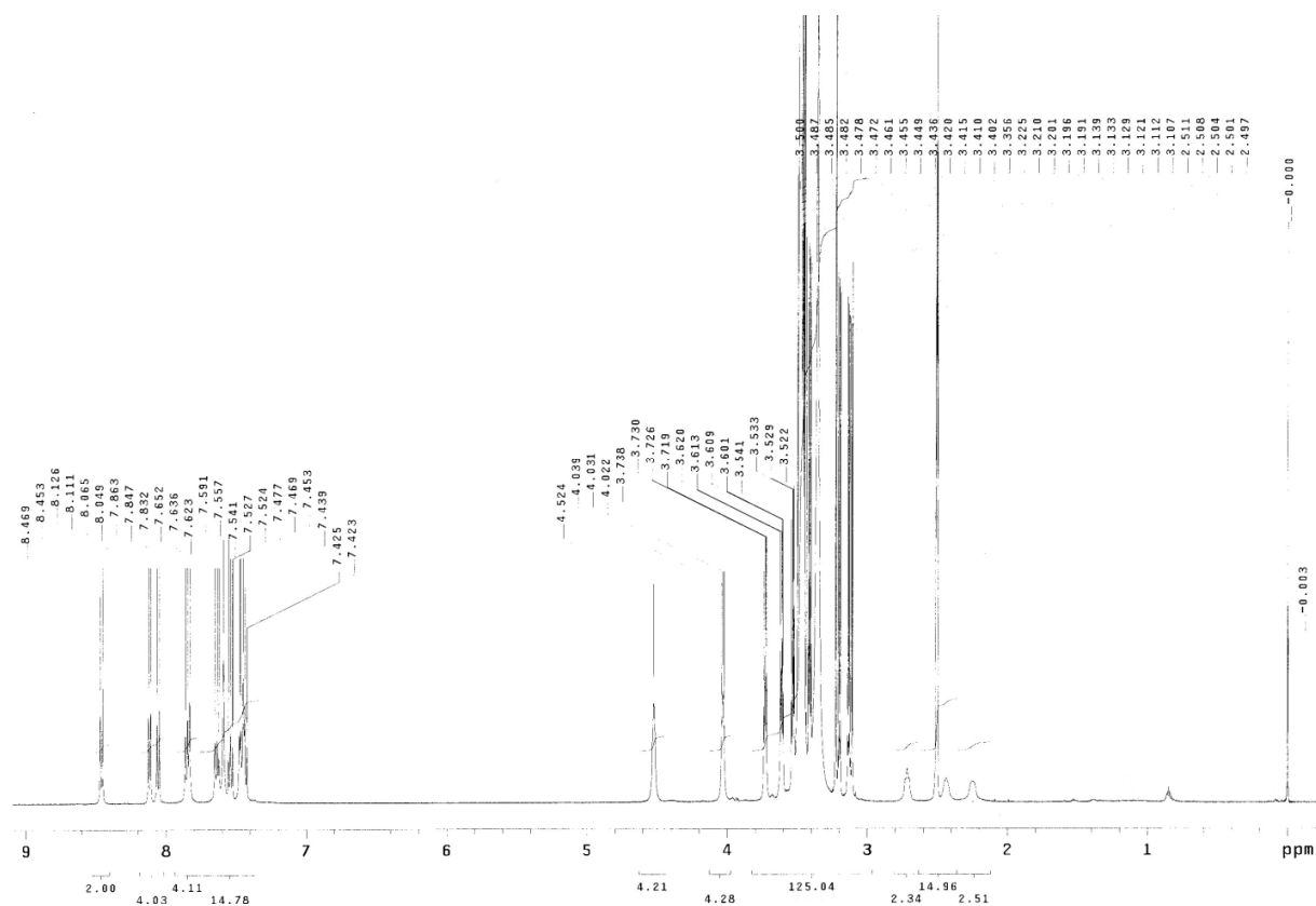
Figure S7. 1 H NMR of compound 1 in d -DMSO.
