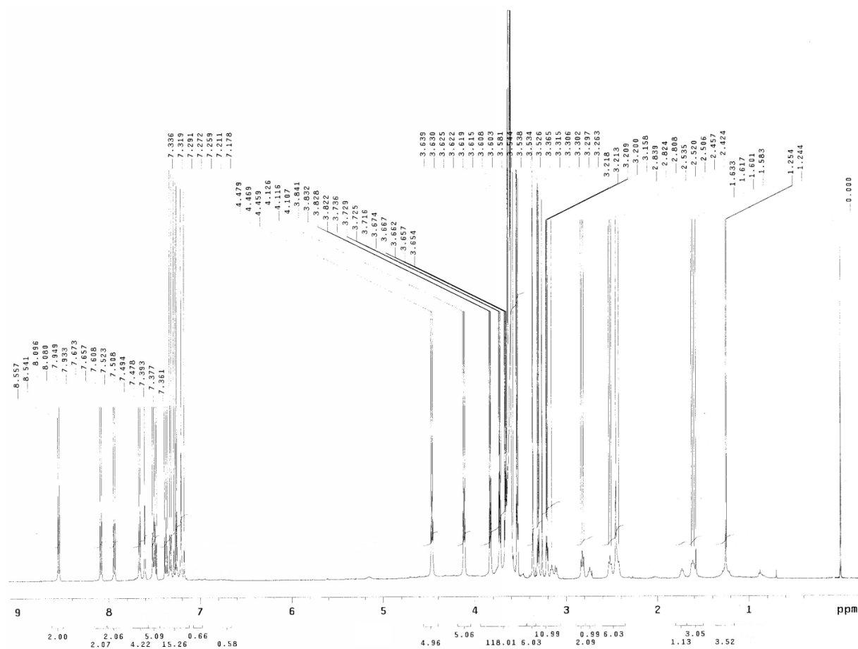
Figure S9. 1 H NMR of compound 2 in CDCl 3 .
