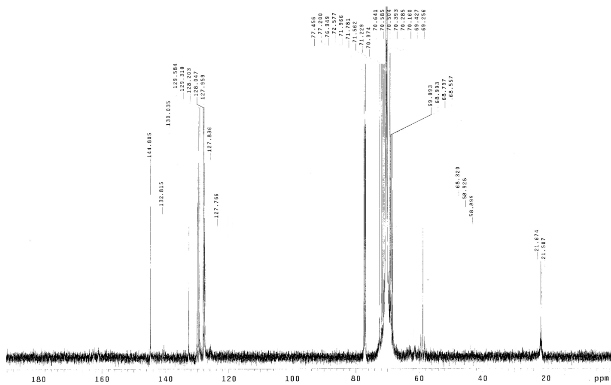
Figure S2. ^{13}\text{C} NMR of compound A in \text{CDCl}_3 .
