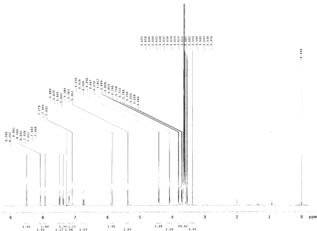
Figure S5. 1 H NMR of compound D in CDCl 3 .
