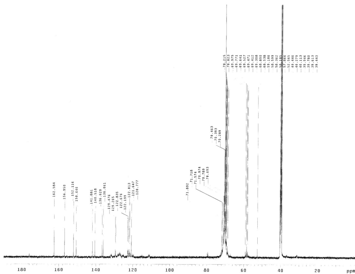
Figure S8. 13 C NMR of compound 1 in d -DMSO.
