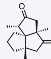
18 NOESY
